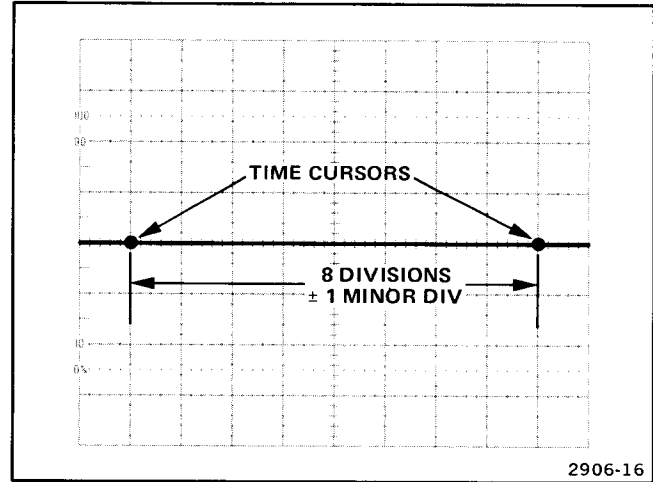
Figure 16. TIME cursor accuracy.
