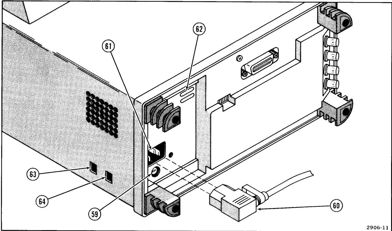
Figure 11. Rear panel and right side panel power controls, connectors, and indicators.
