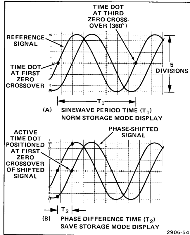
Figure 25. Phase difference between sinusoidal signals.
