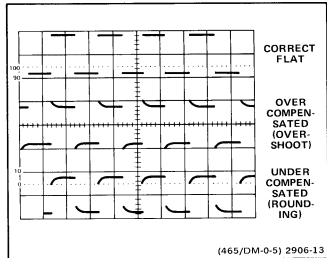
Figure 13. Probe compensation.
