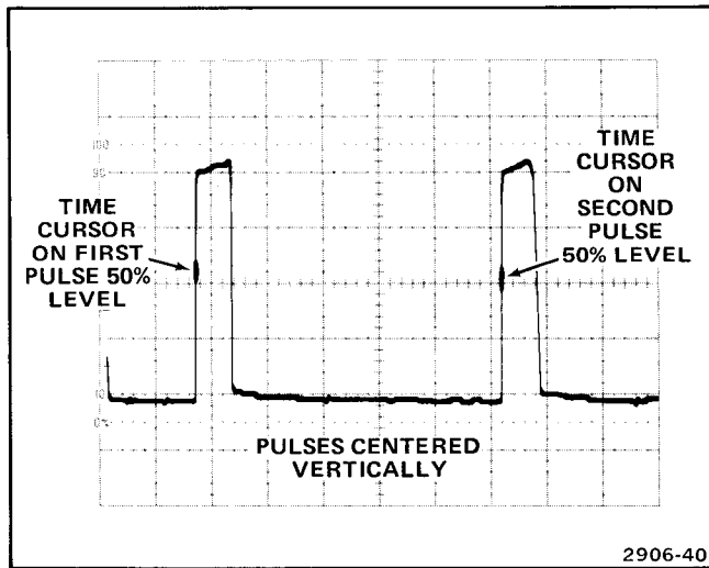
Figure 23. Time difference between repetitive pulses.
