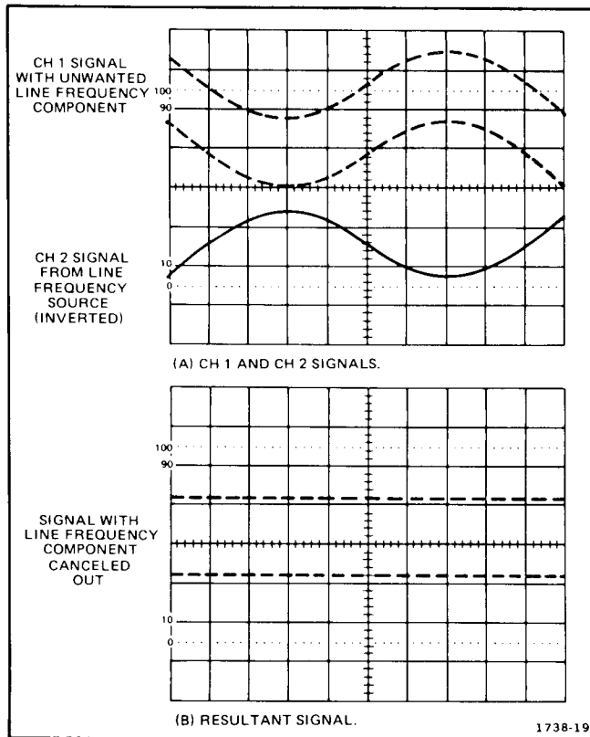
Figure 36. Common-mode rejection.
