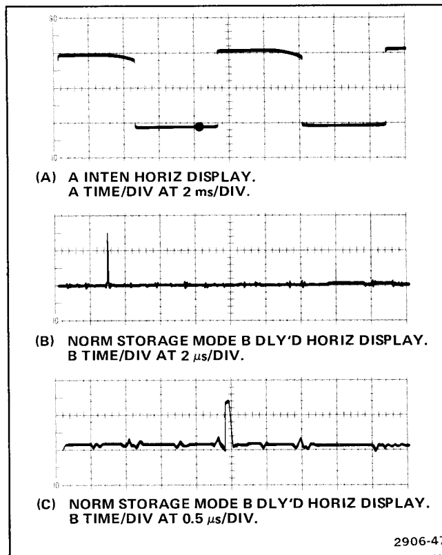
Figure 31. Glitch display, NORM Storage Mode using B DLY'D HORIZ DISPLAY.
