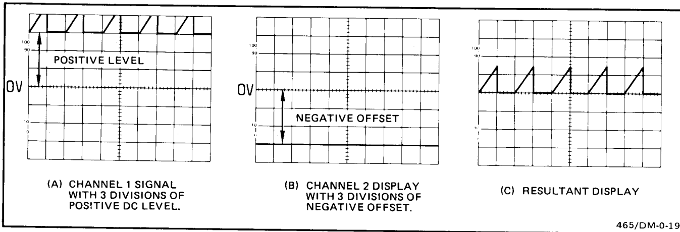
Figure 35. Algebraic addition.
