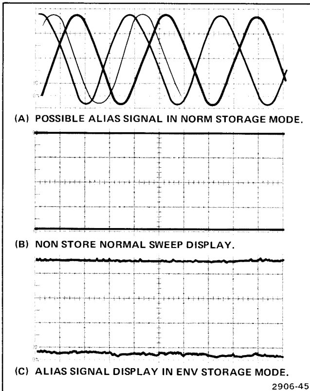
Figure 29. Anti-aliasing.
