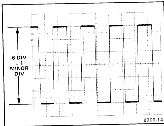
Figure 14. Vertical display accuracy.
